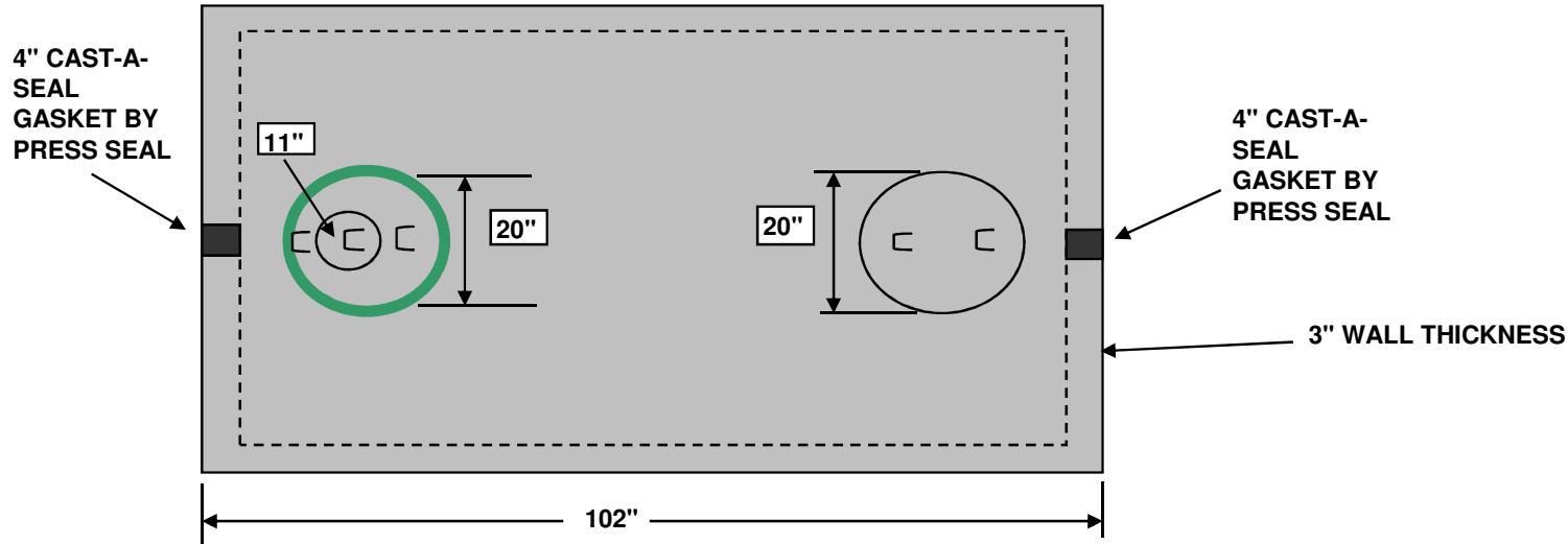
TOP VIEW
