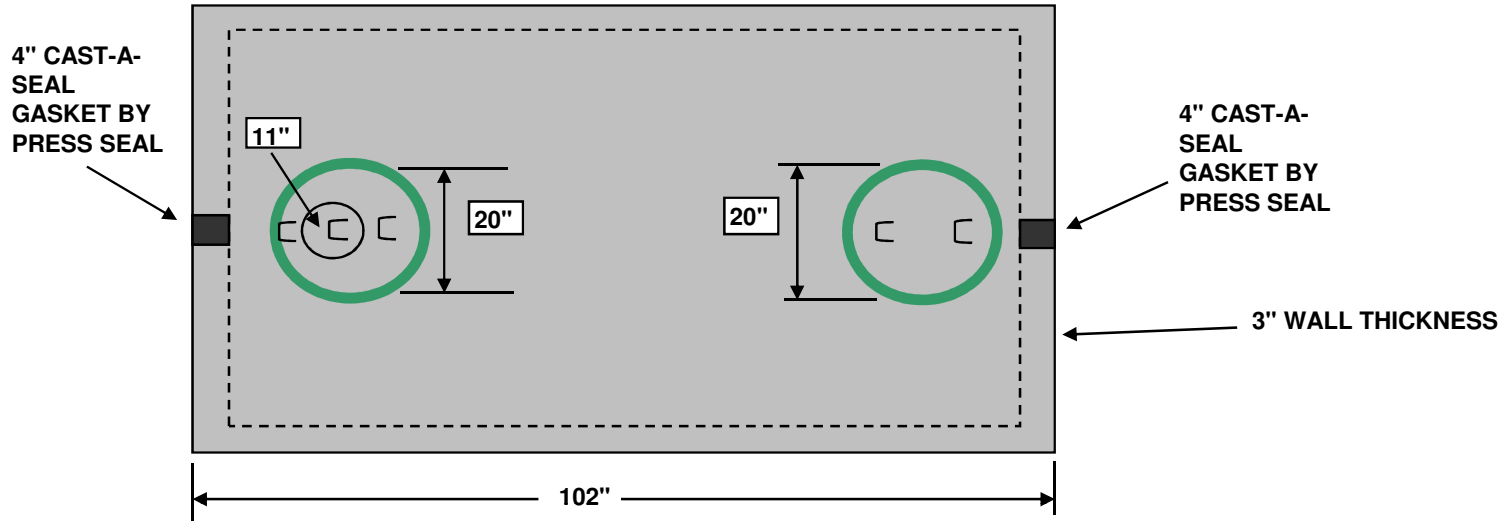
TOP VIEW
