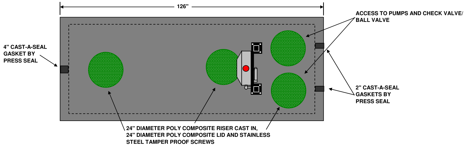
TOP VIEW
