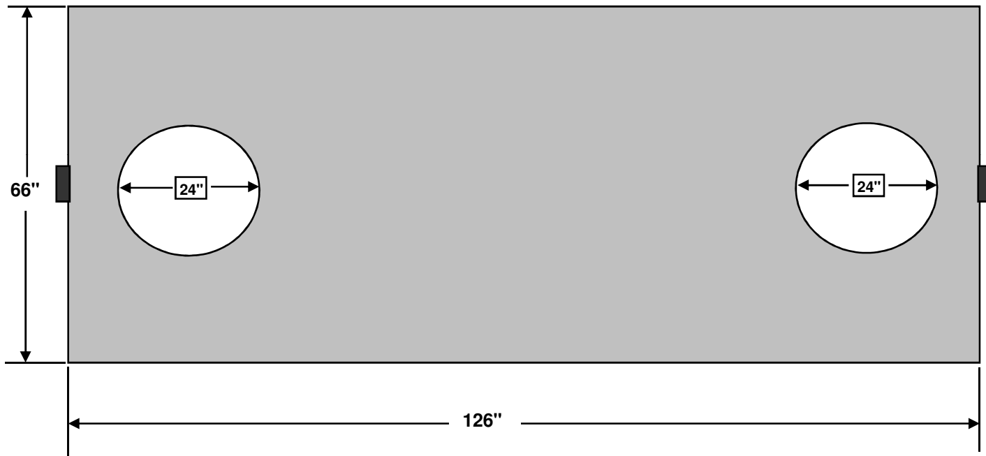
TOP VIEW
