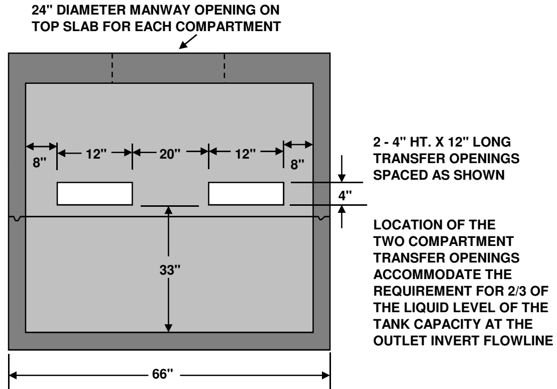
END VIEW CUT AWAY
