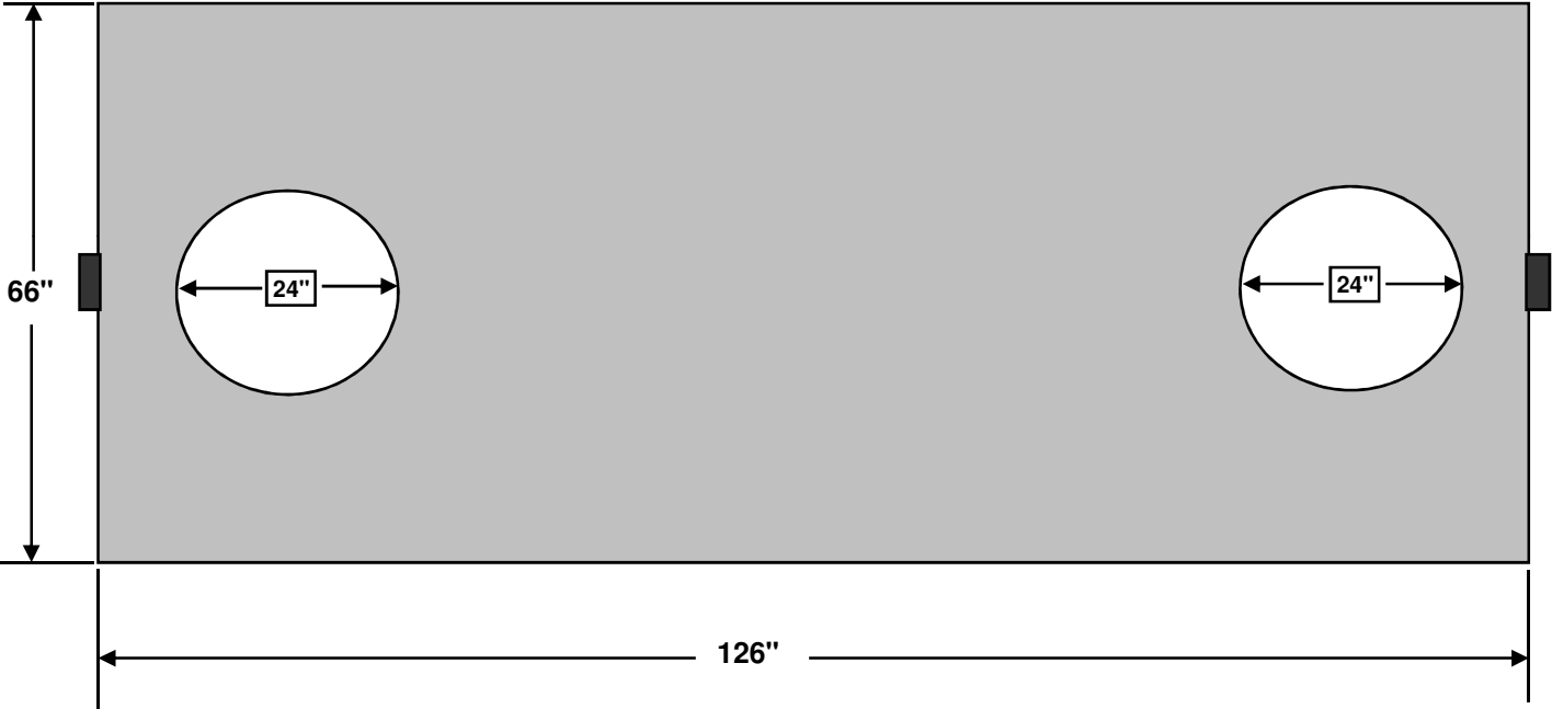
TOP VIEW
