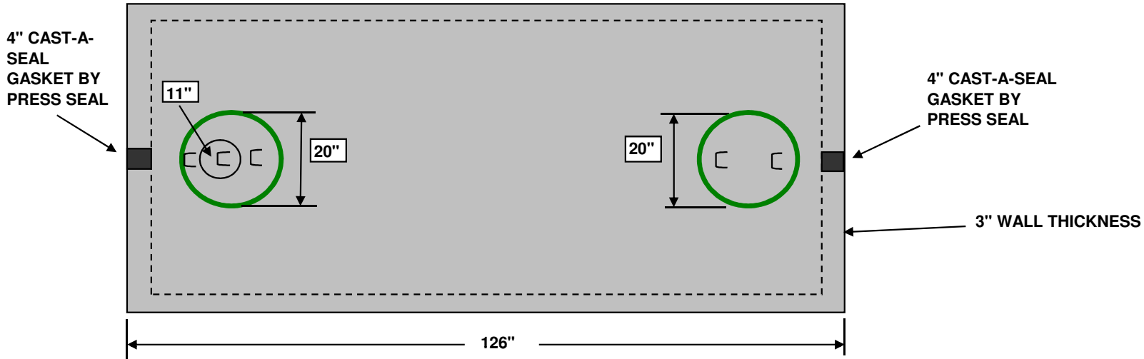
TOP VIEW
