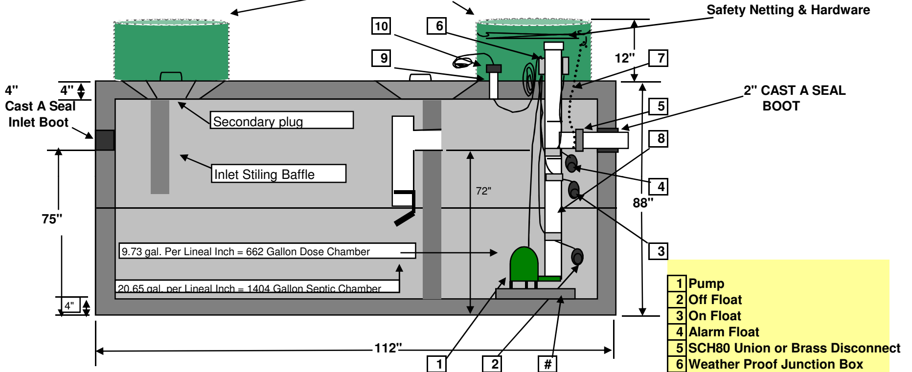
SIDE VIEW CUT AWAY
