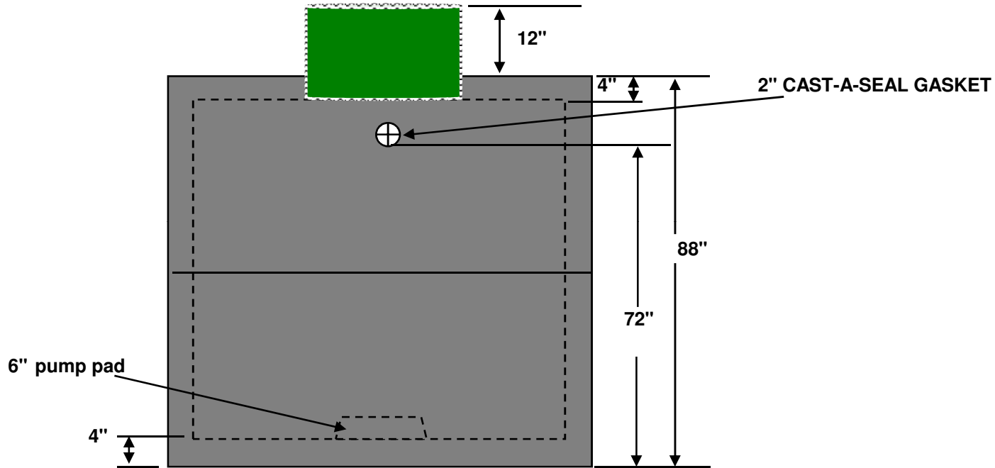
OUTLET END VIEW
