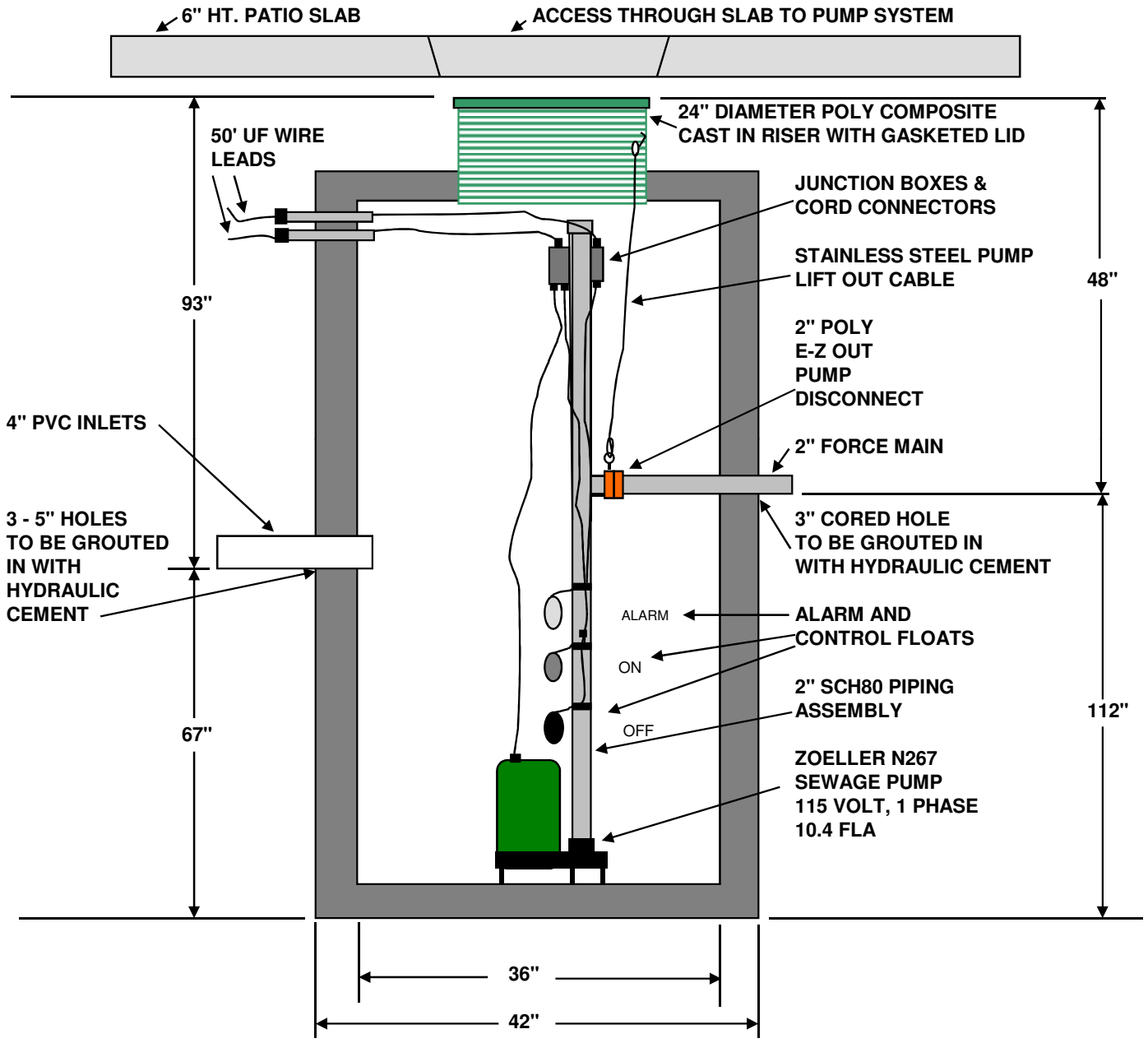
SIDE VIEW CUT AWAY
