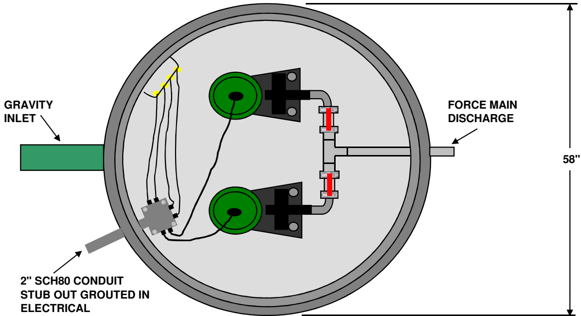
TOP VIEW NO LID
