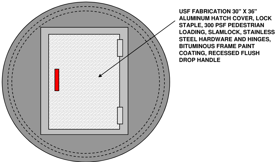
TOP VIEW WITH HATCH COVER
