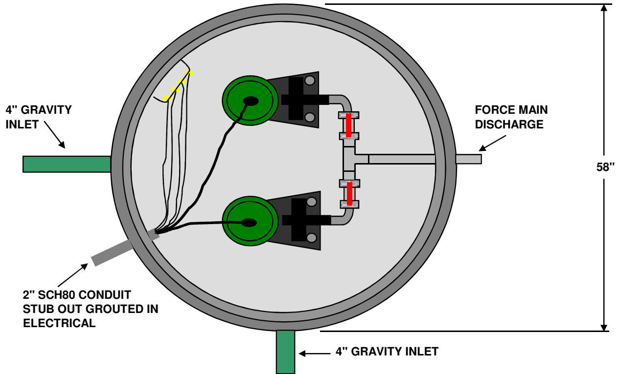
TOP VIEW WITH HATCH COVER
