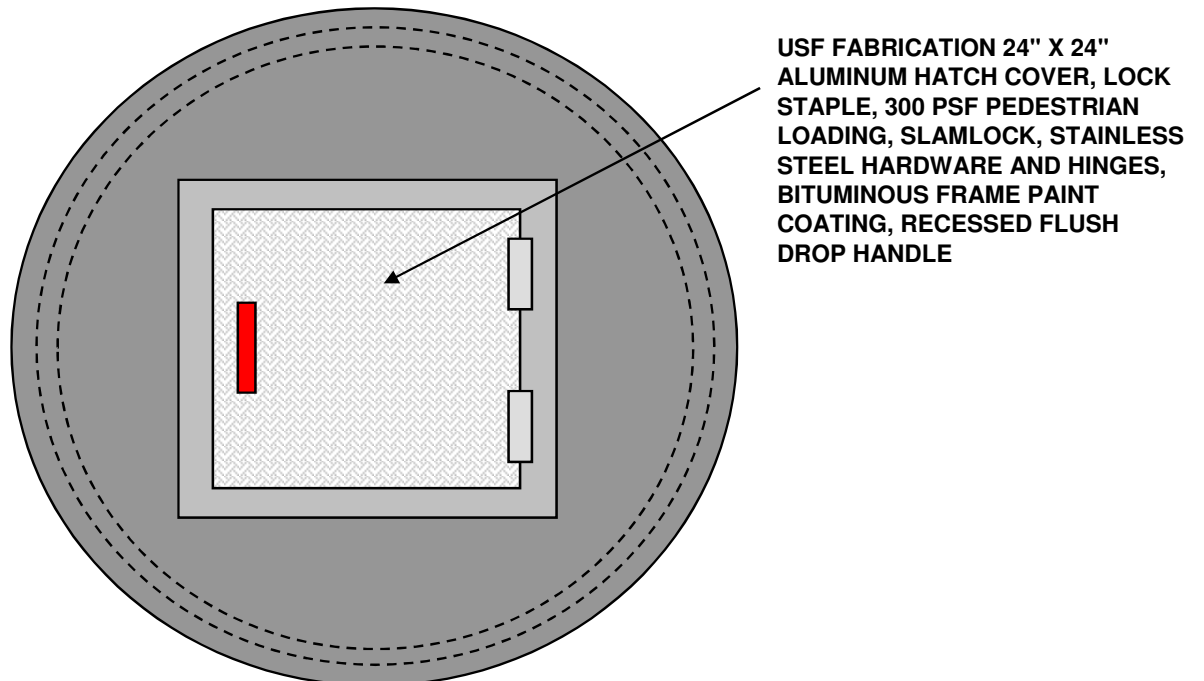
TOP VIEW WITH HATCH COVER
