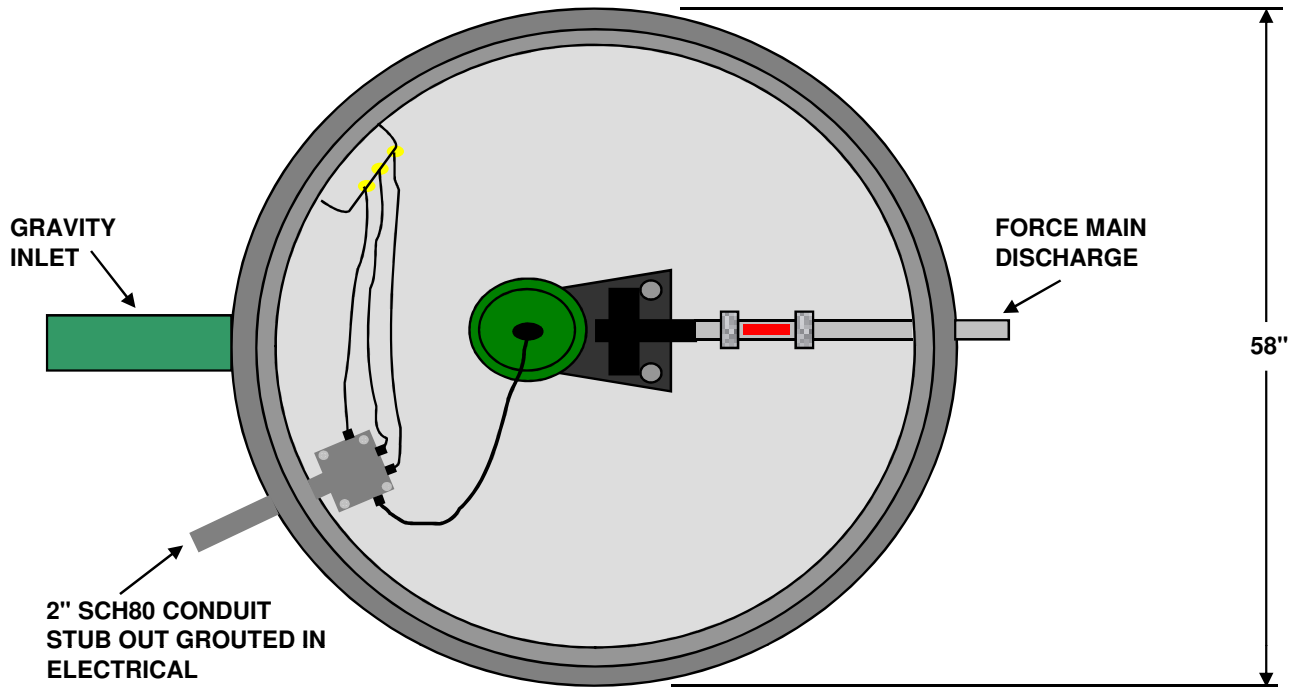
TOP VIEW NO LID
