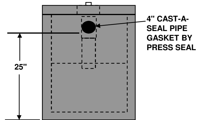
INLET END VIEW
