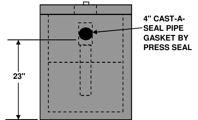
OUTLET END VIEW
