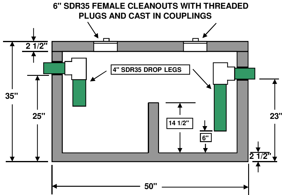
SIDE VIEW CUT AWAY
